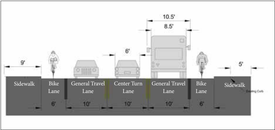
This image shows the proposed street design and dimensions for the section of SE Foster 84th to 89th Avenues compared to the dimensions for a typical TriMet bus and private vehicles.
