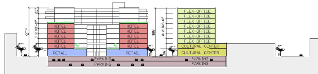
Section A looking north at East Burnside.
