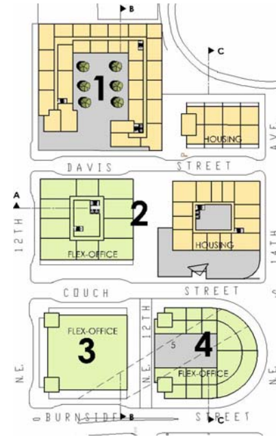
Typical Upper Floor Plan.
